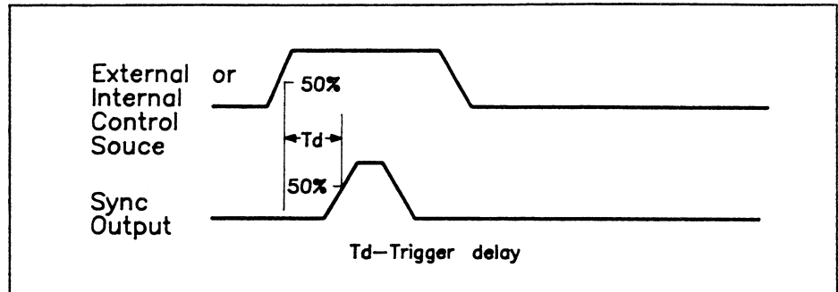
Figure 2-8. Trigger Delay Time for the Sync Output.
