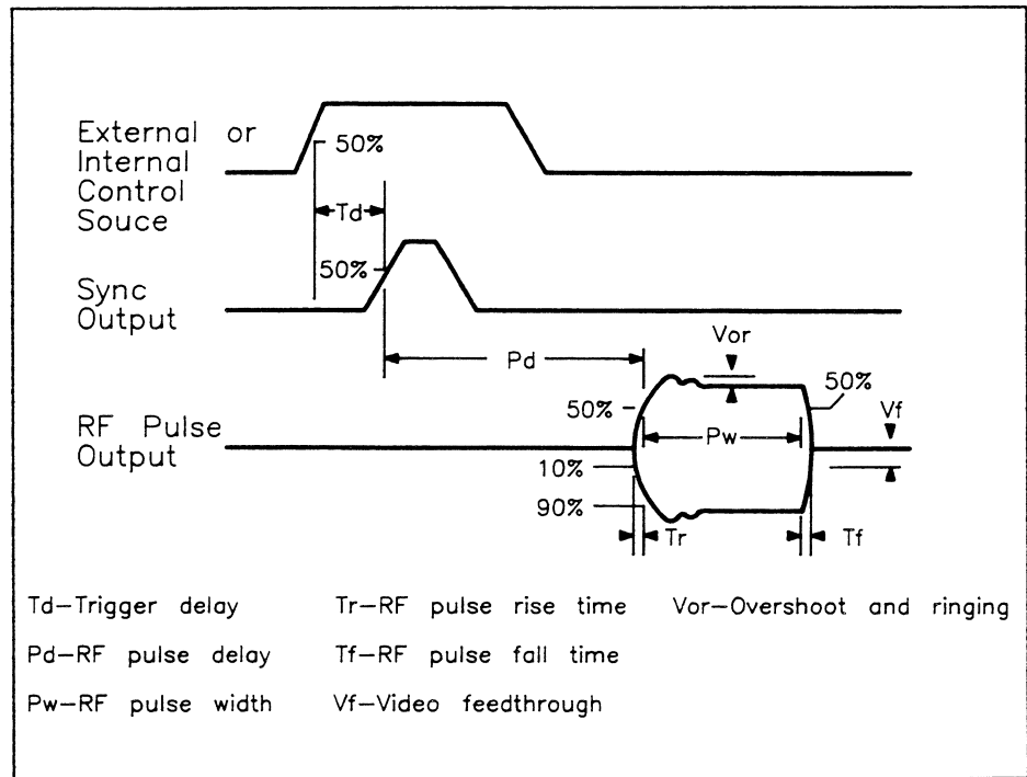
Figure 2-9. RF Pulse Output Characteristics.
