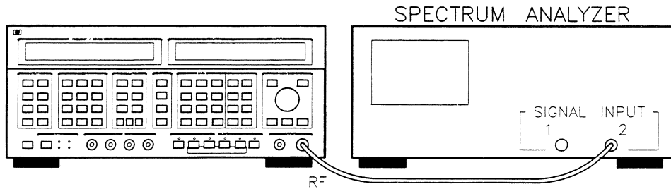
Figure 2-3. Equipment Setup for FM Procedure #1.
