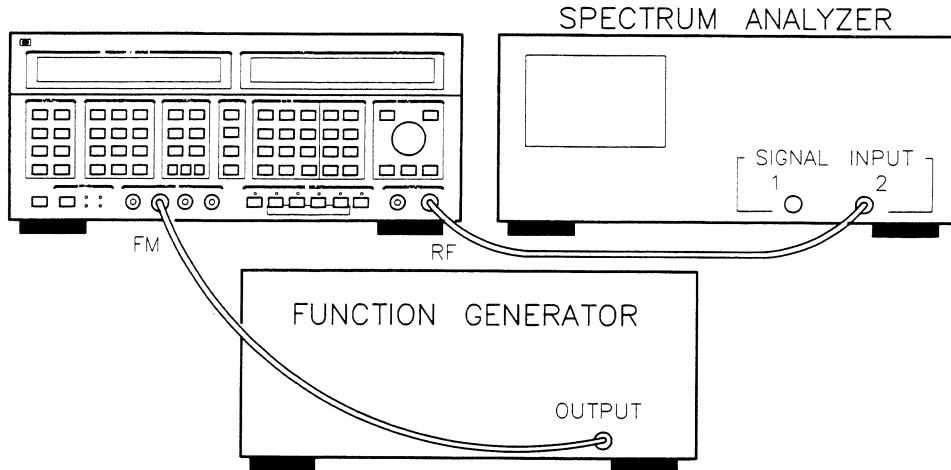
Figure 2-4. Equipment Setup for FM Procedure #2.
